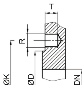
DN 450
